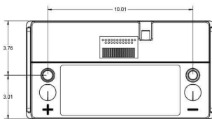
ODP-AGM31A LEFT POSITIVE SAE TERMINALS
