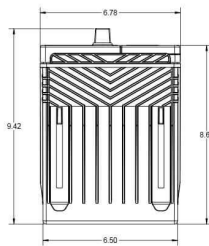
ODP-AGM31A LEFT POSITIVE SAE TERMINALS
