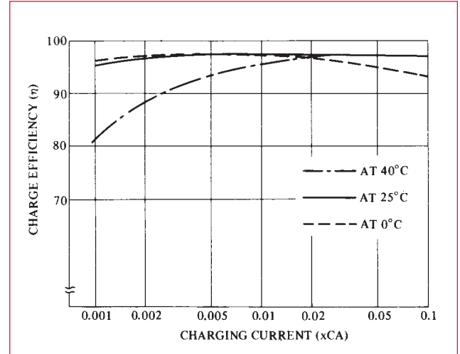
Figure 14. Charging Efficiency
