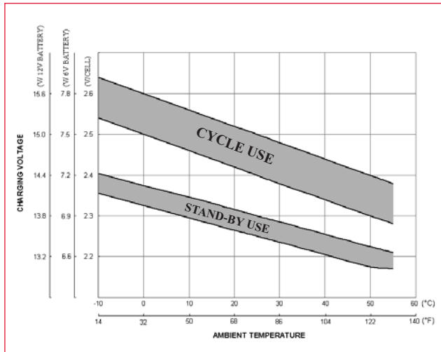
Figure 12. Relationship Between Charging Voltage and Temperature
