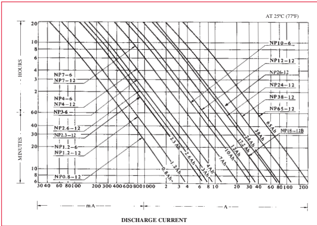
Figure 1. 20-Hour Rate Capacity Selection Chart
